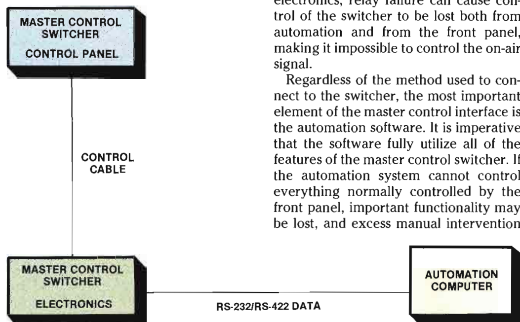
Figure 1. A master control switcher with a serial port is the easiest to automate.
