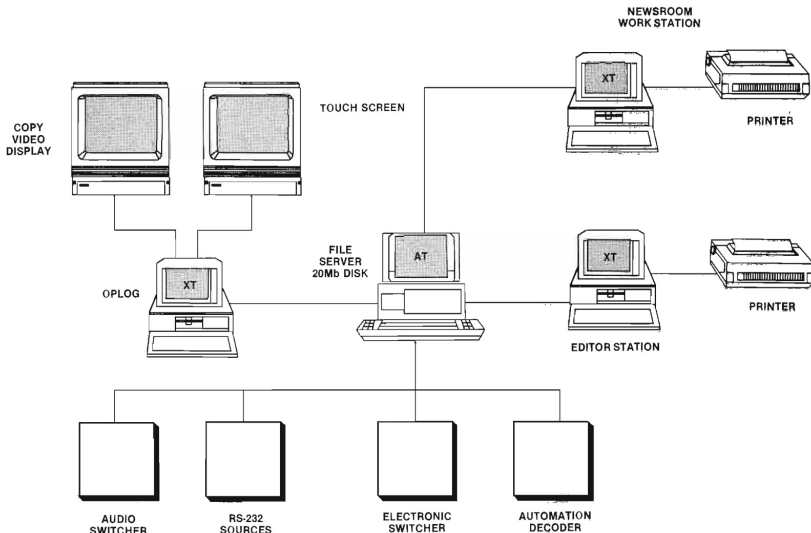
Figure 1. the heart of the Media Touch system is the software residing in the file-server computer. This computer controls the RS-232 bus and directs data between the other devices.
